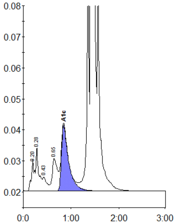
Peak table - ID: 10450726
